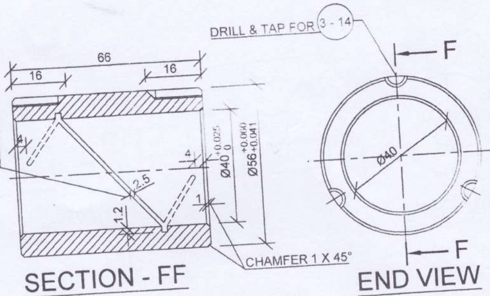
BUSH (3 - 13) (FOR OPERATING ARM)
