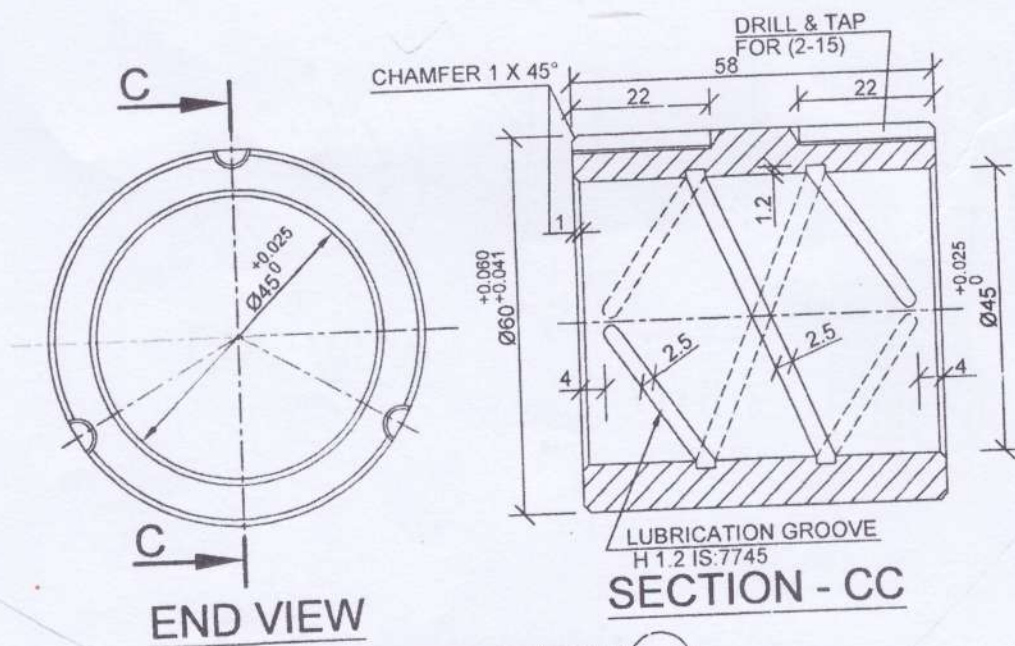
WHEEL BUSH (2-11) MATL. :- LTB - 1 OF IS:318
