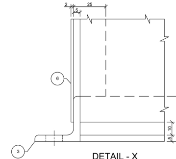
DETAIL - X
