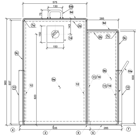
VIEW-CC
