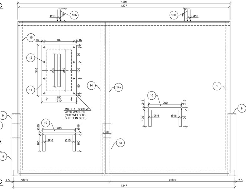
VIEW - CC
