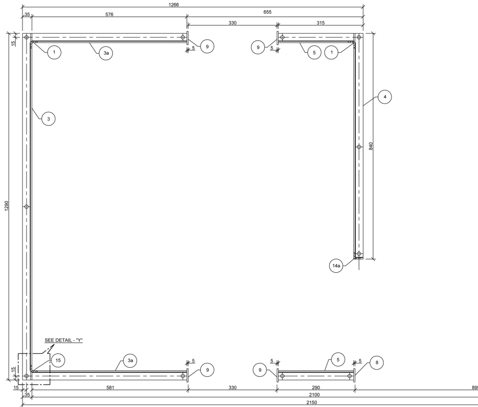
SECTION - AA
