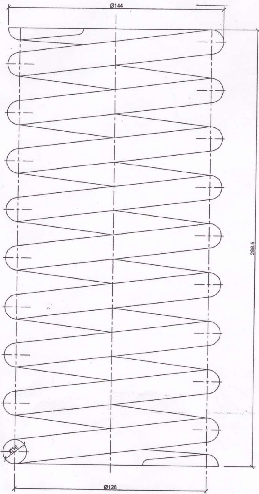
HELICAL COMPRESSION SPRING (17-4)
