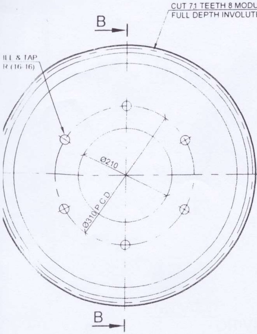
END VIEW
