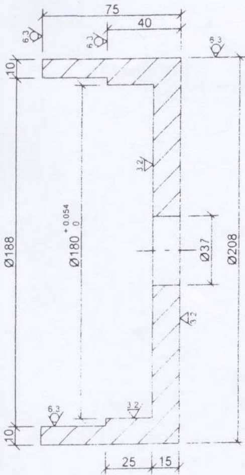
SECTION - CC
