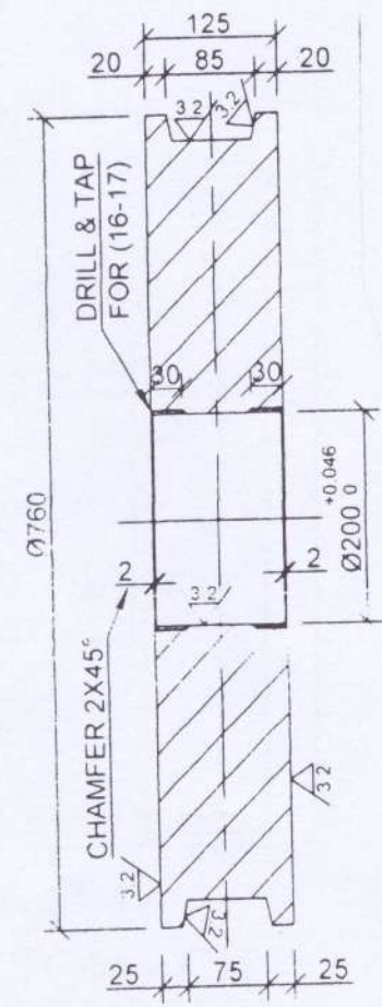
SECTION - EE
