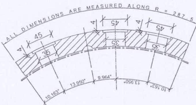
SECTION - FF
