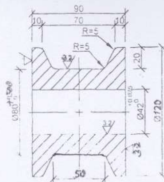
SECTION - NN GUIDE ROLLER (5-10) MATERIAL - 55C8 OF IS.2004
