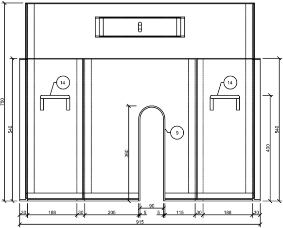
END VIEW
