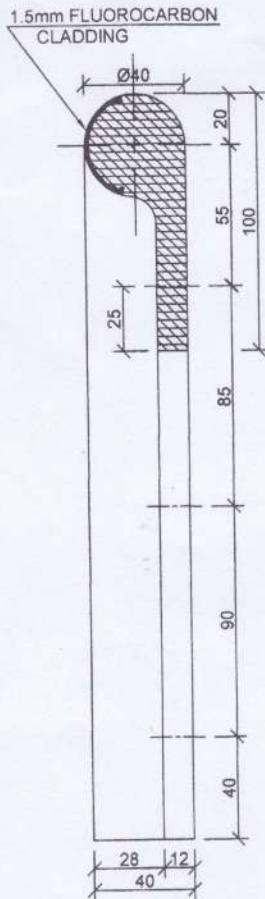
END VIEW
