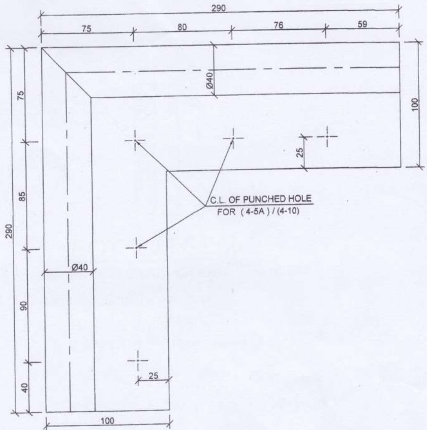
CORNER SEAL (4-9)
