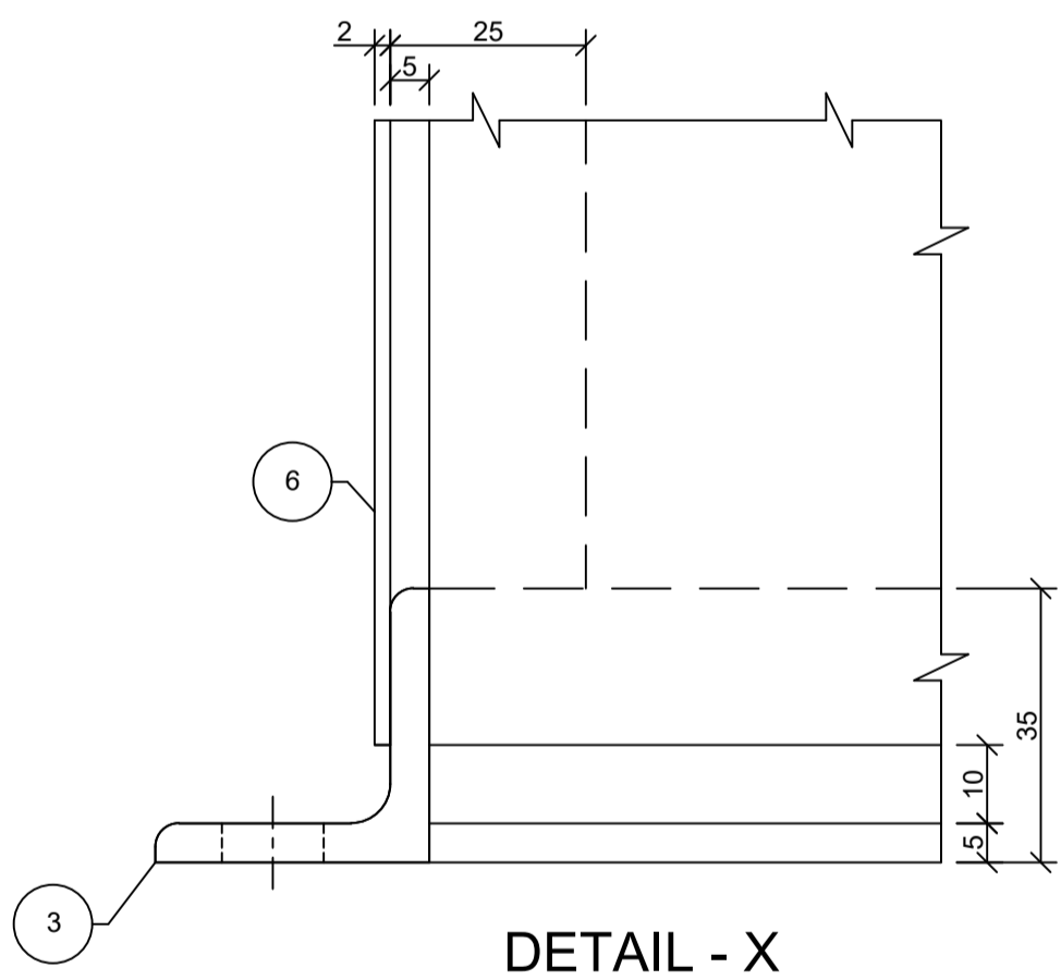
DETAIL - X
