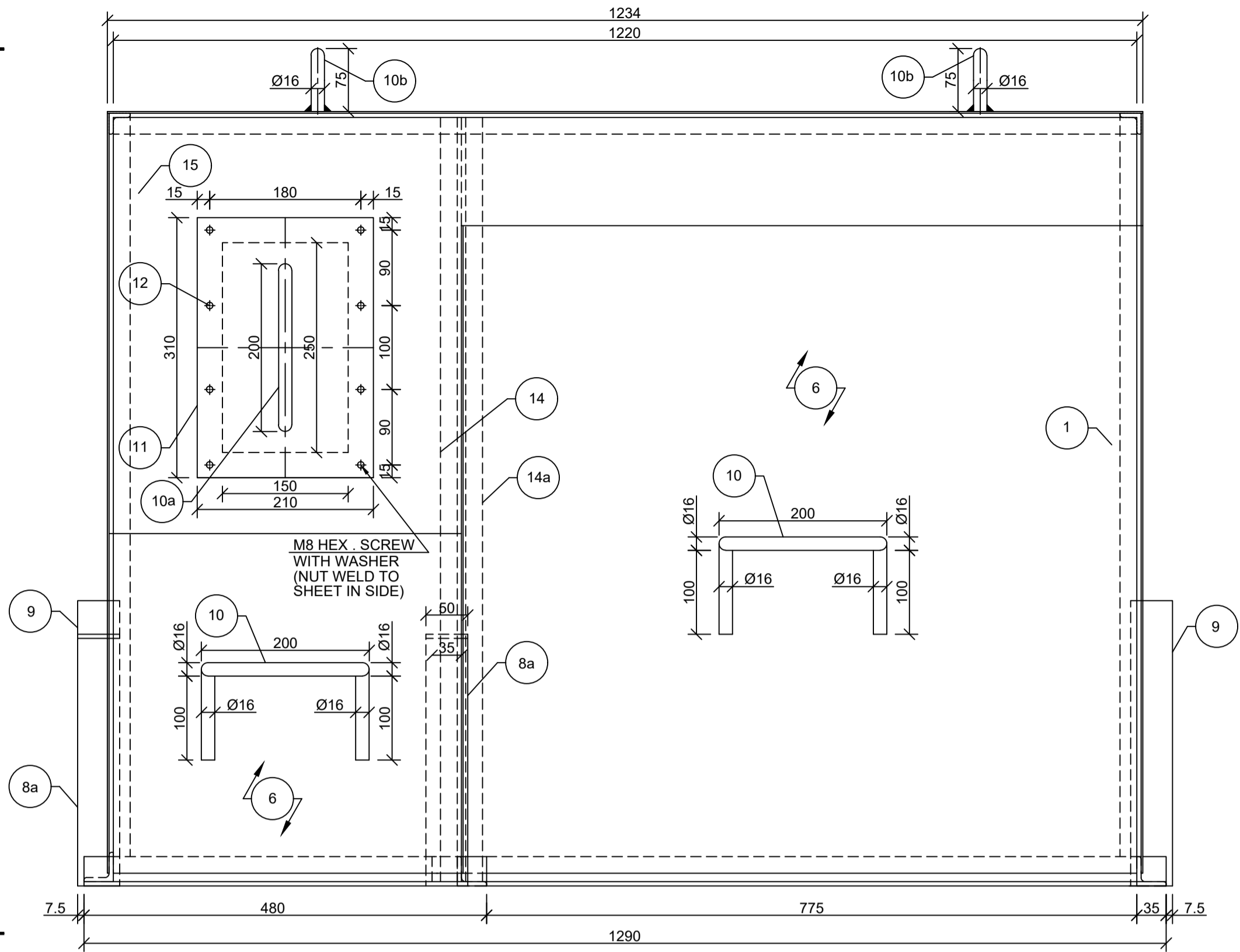
VIEW - CC
