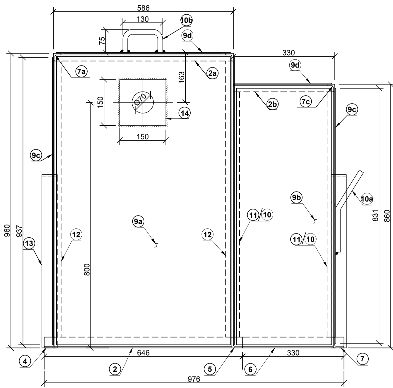
VIEW-CC
