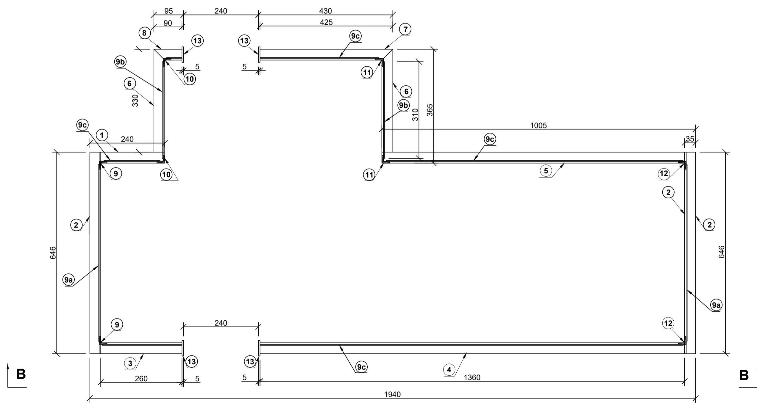
SECTION - AA
