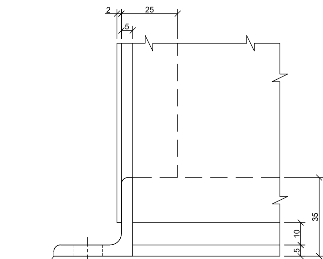
DETAIL - X
