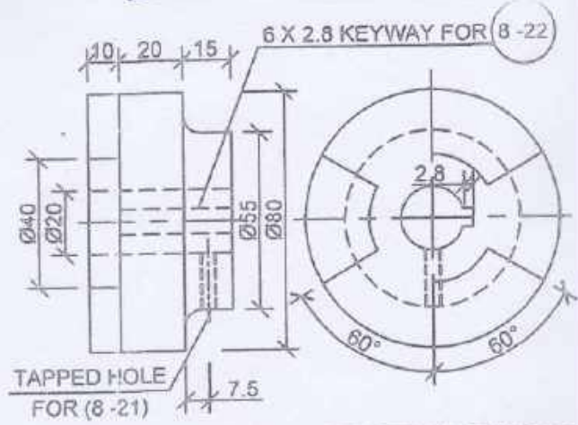
END VIEW ELEVATION
