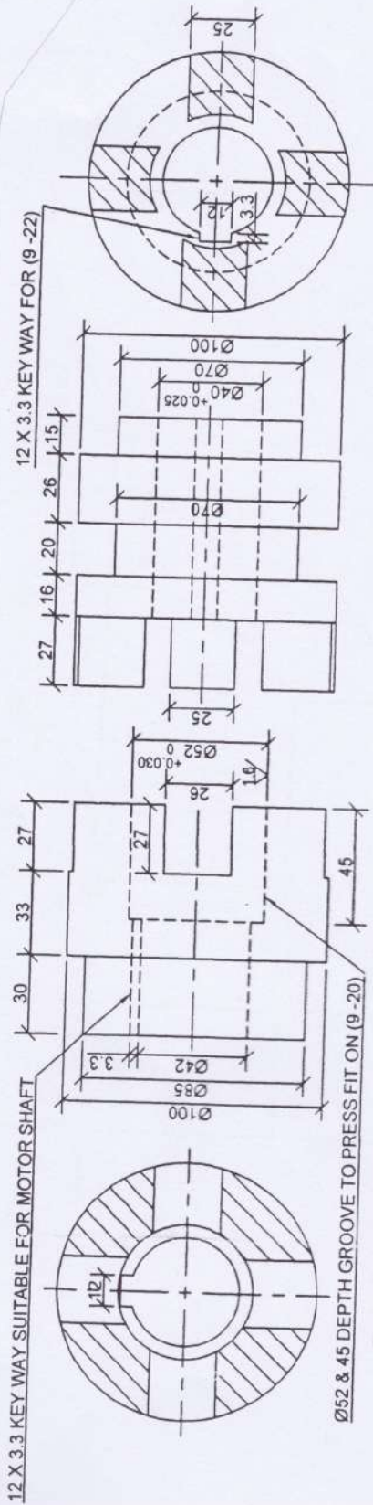
DOG CLUTCH (FIXED) (9-5)
