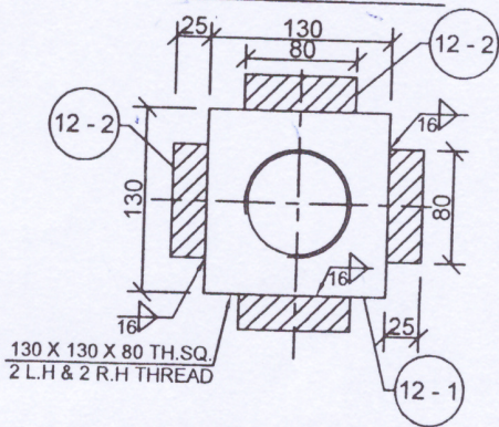
SECTION-CC COUPLER NUT ASSEMBLY
