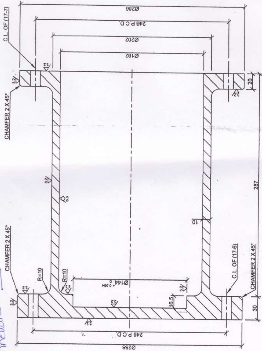
SECTION - BB
