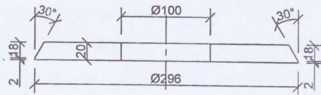
DETAIL OF S.S. PLATE (2)
