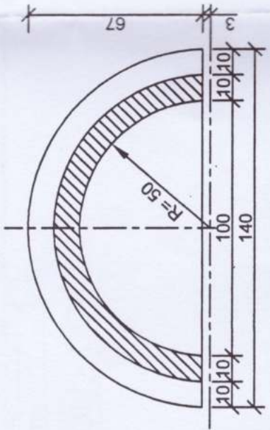
SECTION - MM
