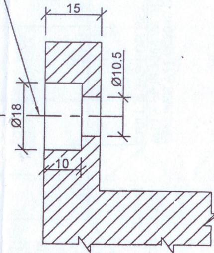
DETAIL - "Y"
