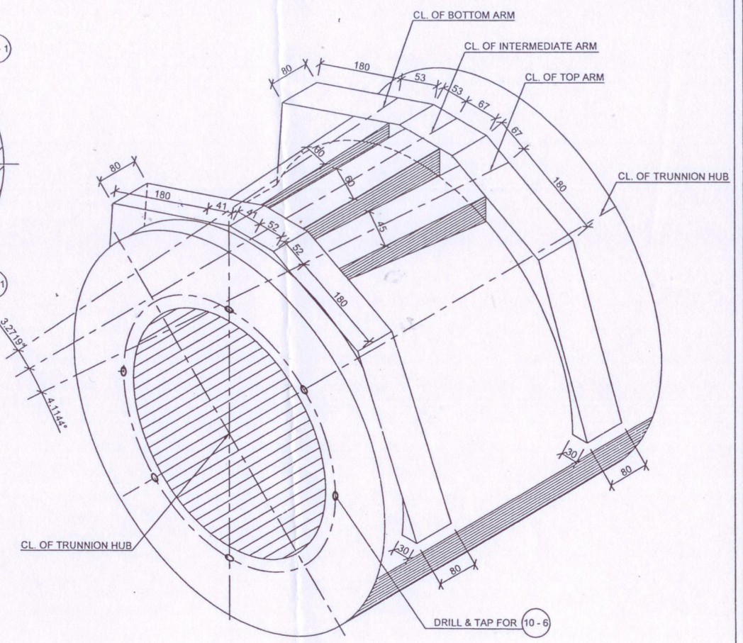
TRUNNION HUB MATERIAL:- CAST STEEL GR.340-570W OF IS:1030-1989 NOS. REQUIRED/SET:- 2 (1L & 1R)
