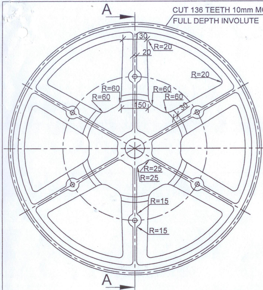
END VIEW
