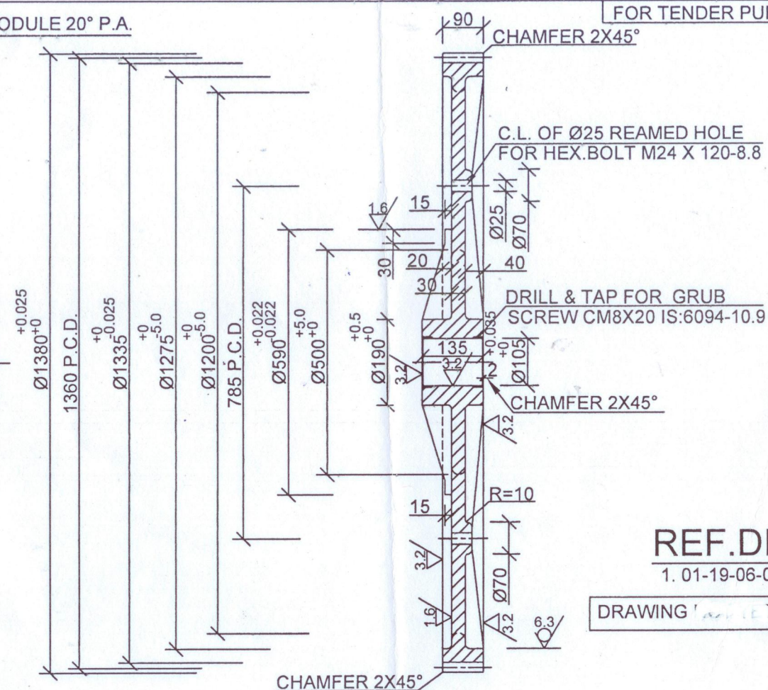
SECTION - AA
