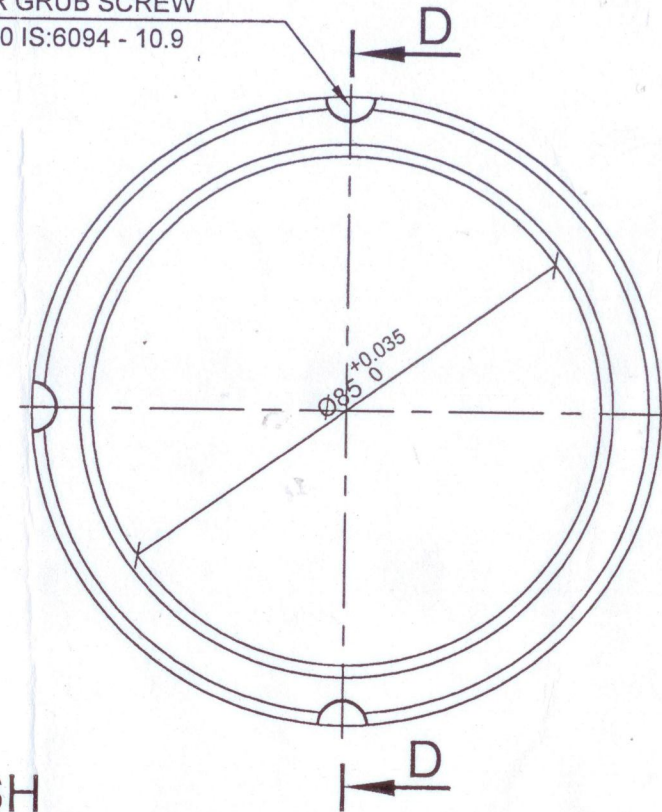
END VIEW
