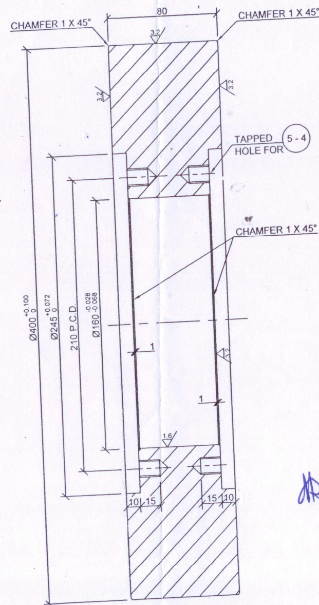
SECTION - AA
