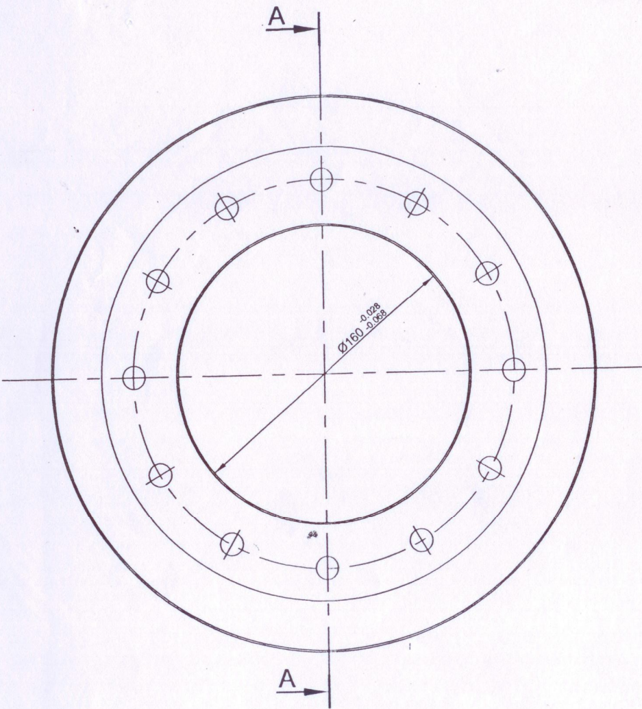
WHEEL (6-1) MATERIAL - 45C8 OF IS:2004
