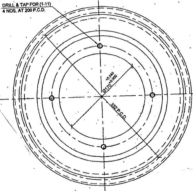
WORM GEAR (1-1)
