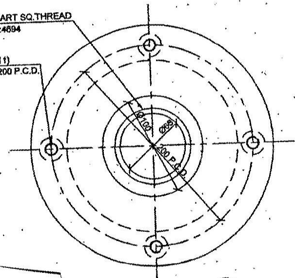
BRONZE NUT (1-10)
