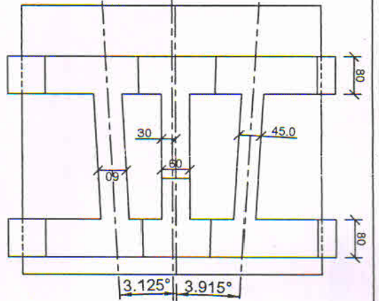
VIEW - BB
